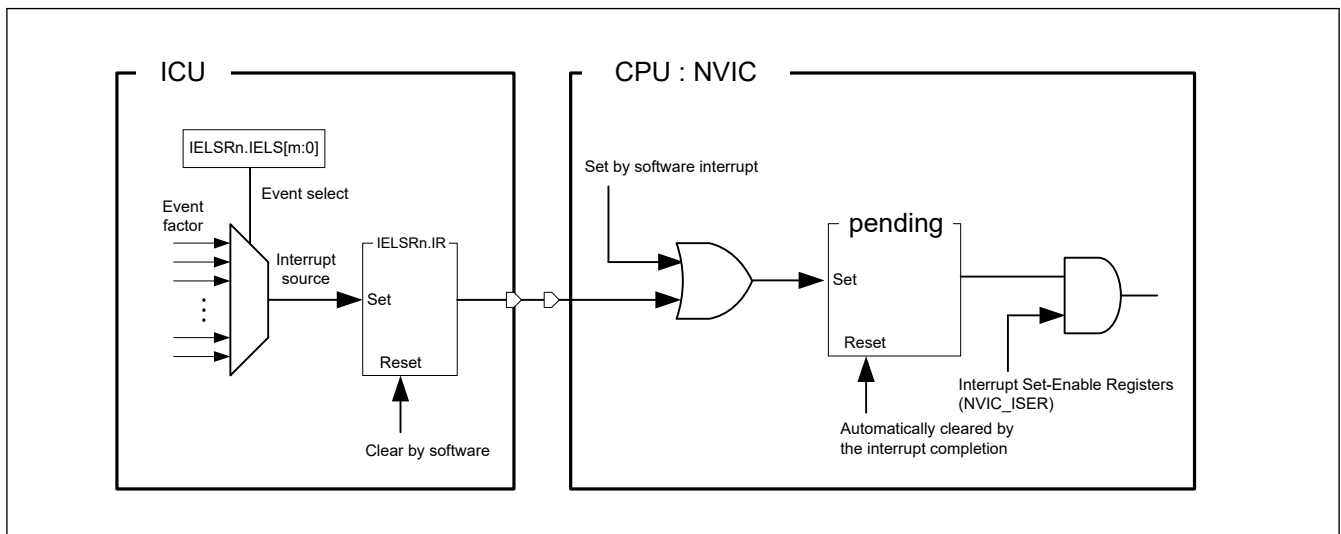
Figure 14.3 Interrupt path of the ICU and CPU : NVIC
